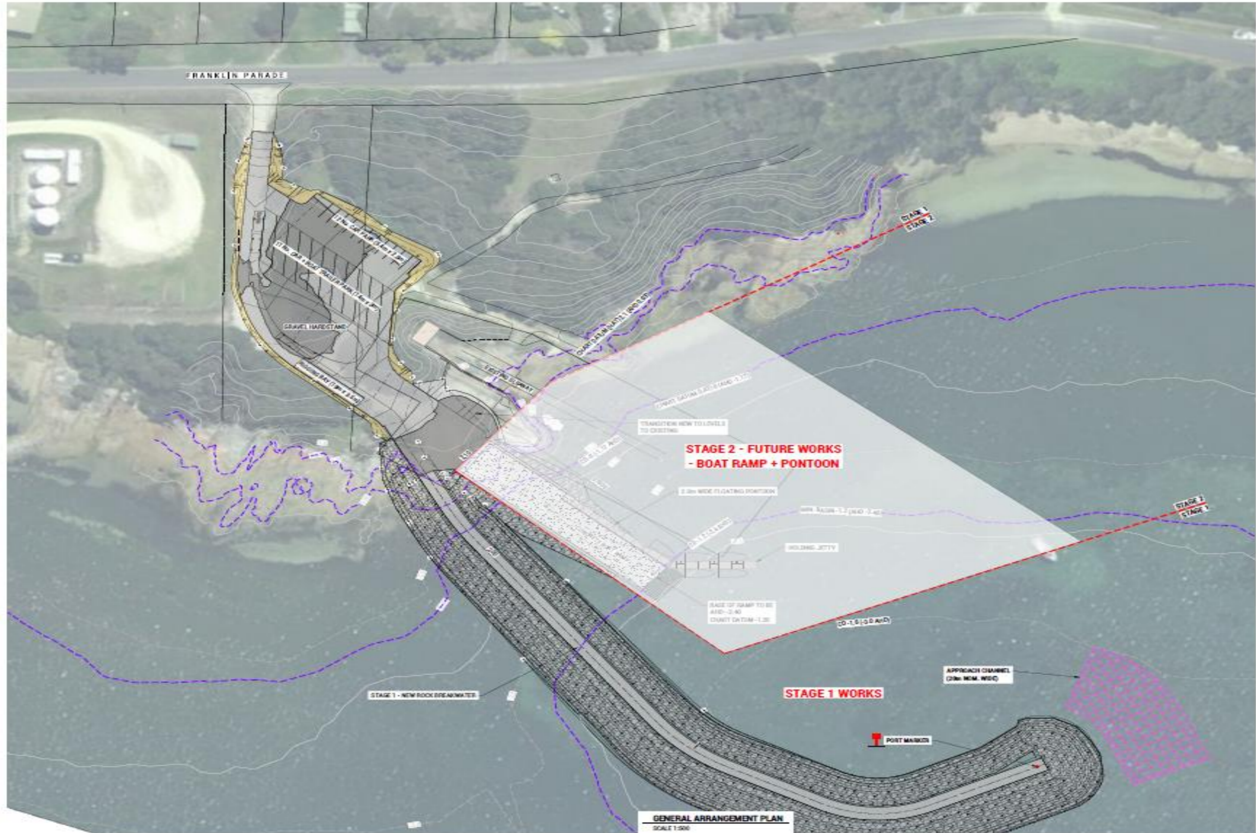
Option 2 extended rock wall alignment (excluding all land-based infrastructure shown in this diagram)
